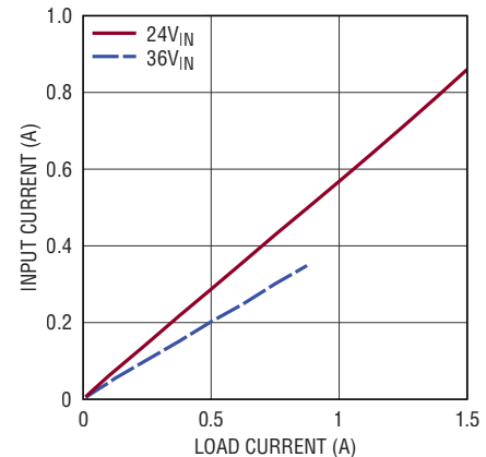
Input vs Load Current V_{OUT} = 12V
