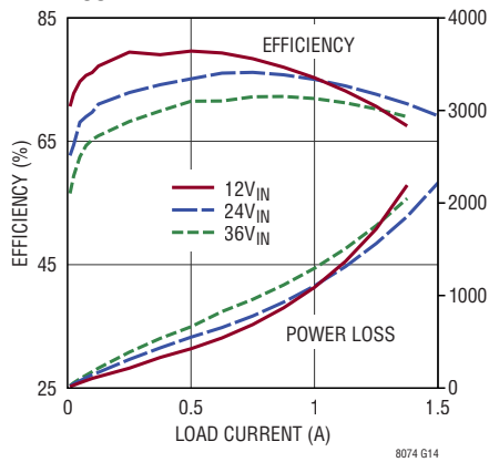
Efficiency and Power Loss, V OUT = -3.3V
