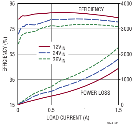
Efficiency and Power Loss, V OUT = 5V, f SW = 2MHz
