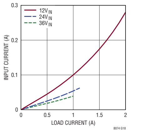
Input vs Load Current, V OUT = 0.8V
