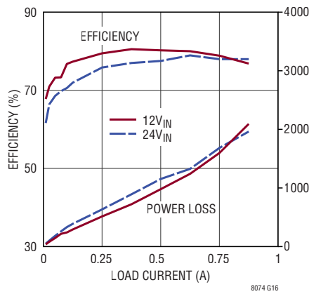
Efficiency and Power Loss, V OUT = -8V
