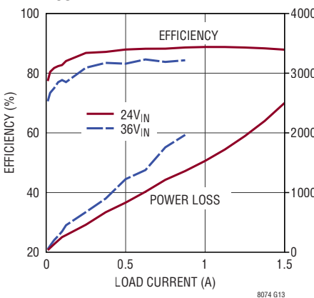
Efficiency and Power Loss, V OUT = 12V
