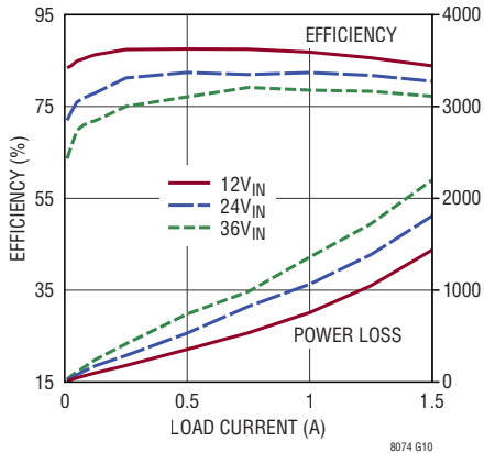
Efficiency and Power Loss, V OUT = 5V
